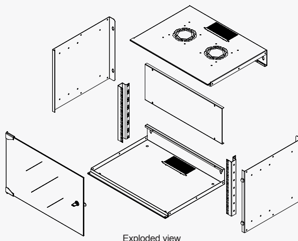
Exploded view
