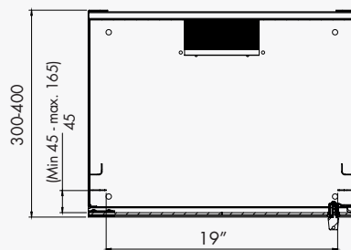
Mounting profile
