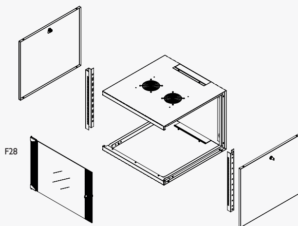
Exploded view
